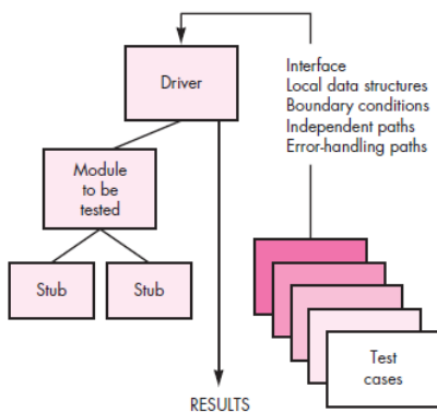
Figure. Unit-test environment
