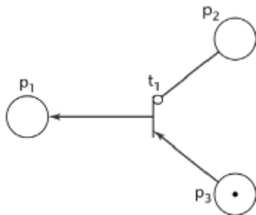
Fig. A petrinet with an inhibitor arc
