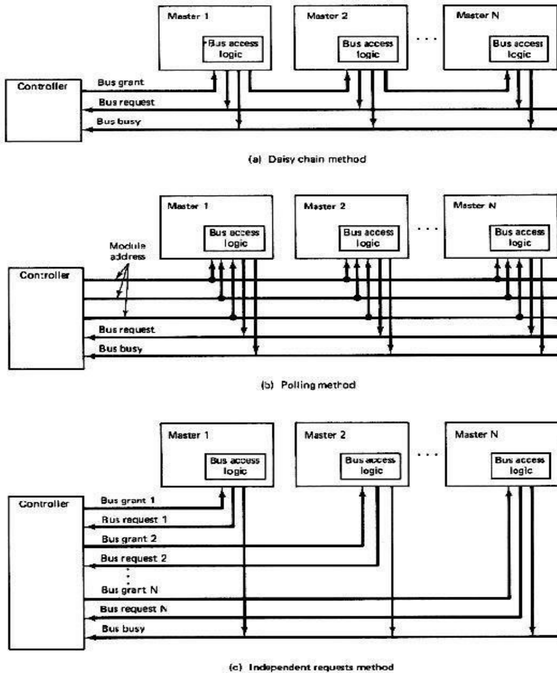
Fig.2.16 Bus allocation schemes
