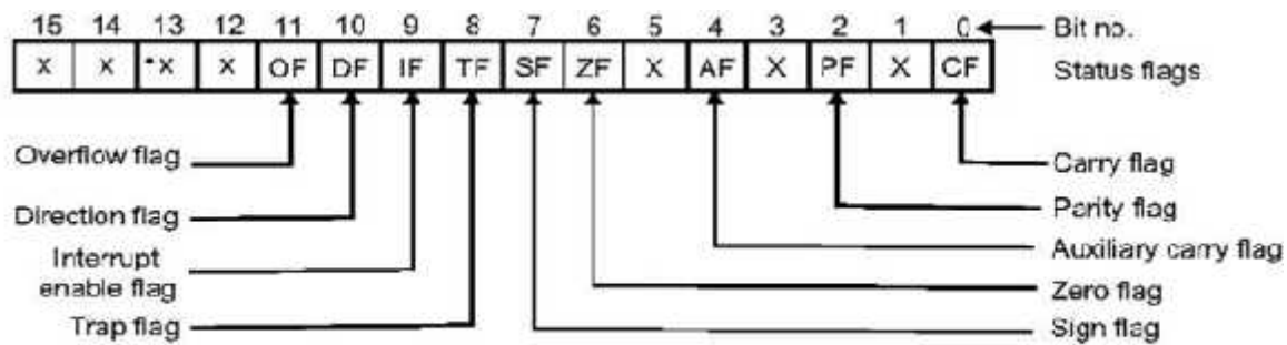
Fig.11.8: Status flags of intel 8086
