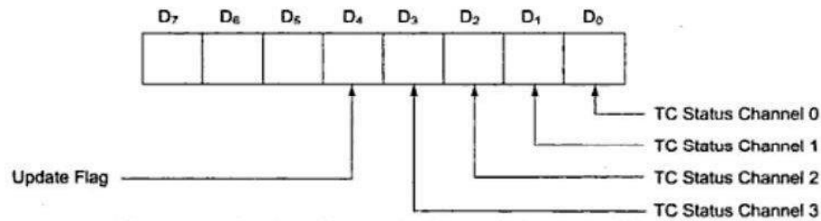
Fig 3.33 Status Register
