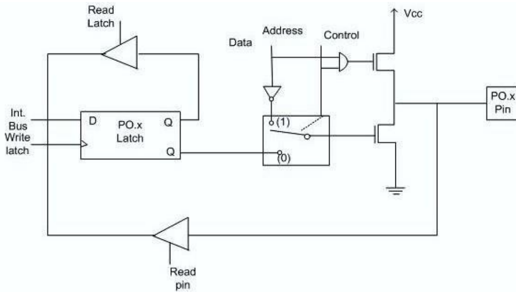
Fig 4.6 Port-0 Structure
