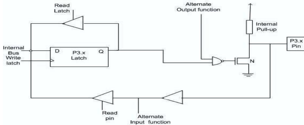
Fig. 4.9 Port 3 structure
