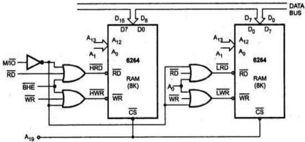
Fig 3.5 Block decoding
