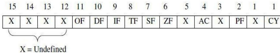
Fig. 1.5 Flag Register
