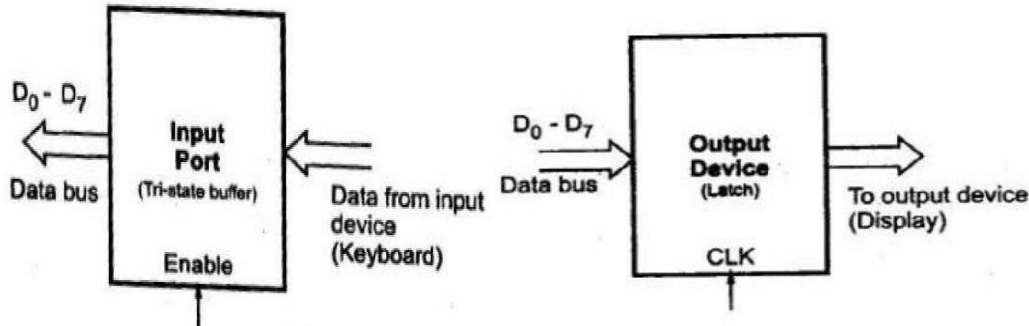
Fig.3.7 I/O interfacing
