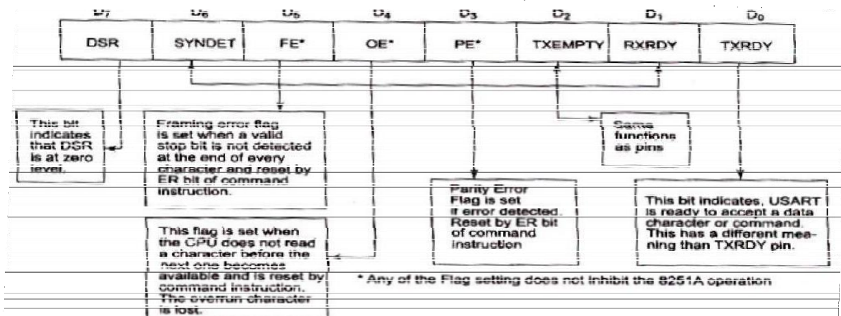
Fig. 3.20 Status information
