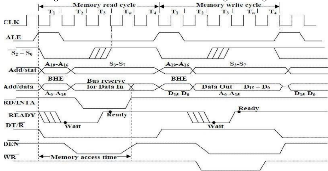
Fig.2.2. General Bus operation cycle
