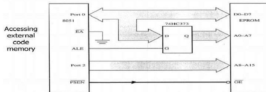
Fig. 5.6 External Memory interfacing
