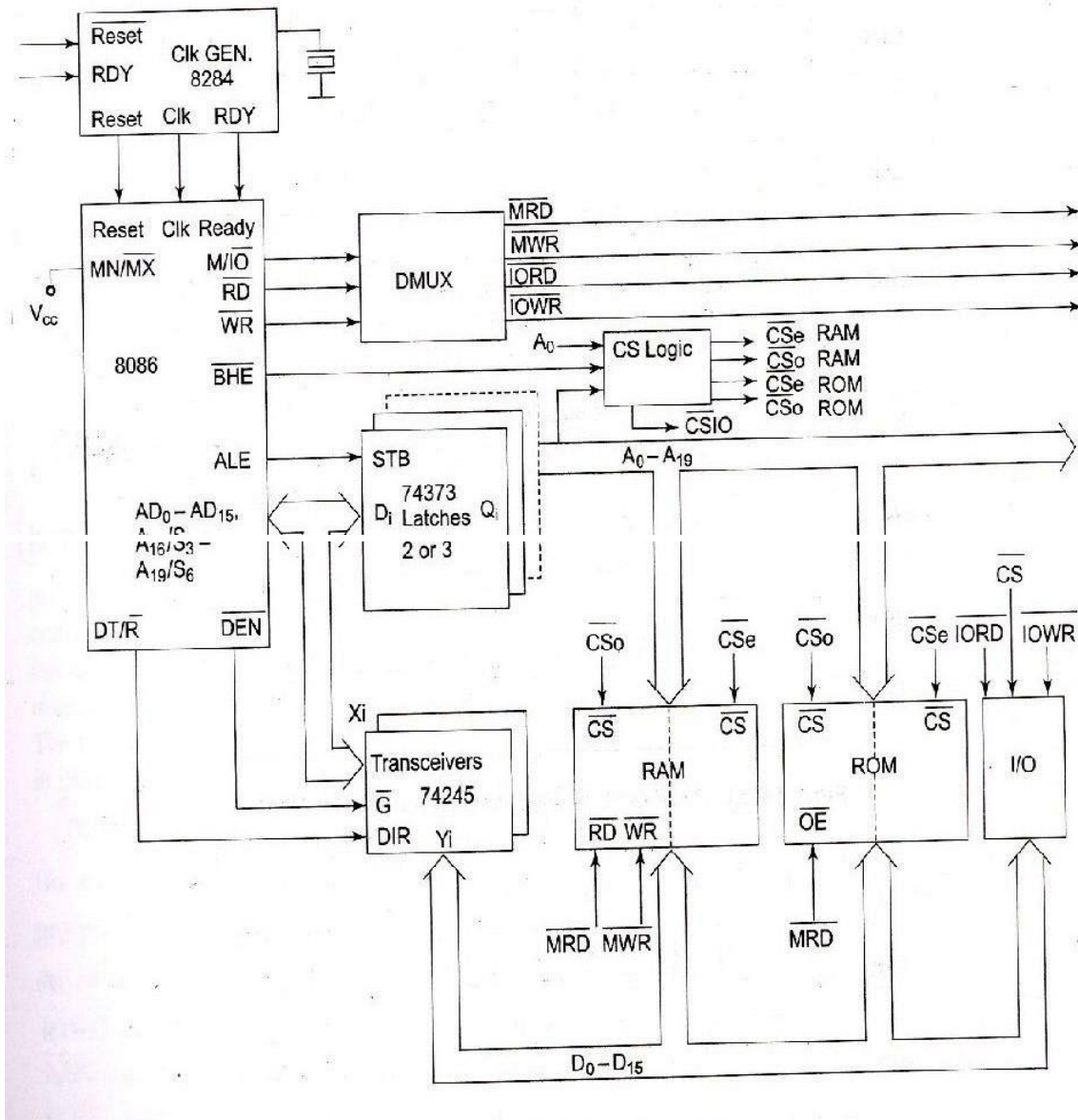
Fig 2.3. Minimum Mode 8086 System
