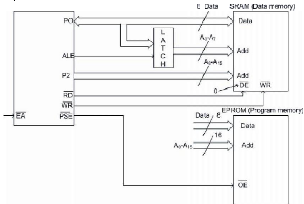
Fig 4.10 Circuit Diagram for Interfacing of External Memory
