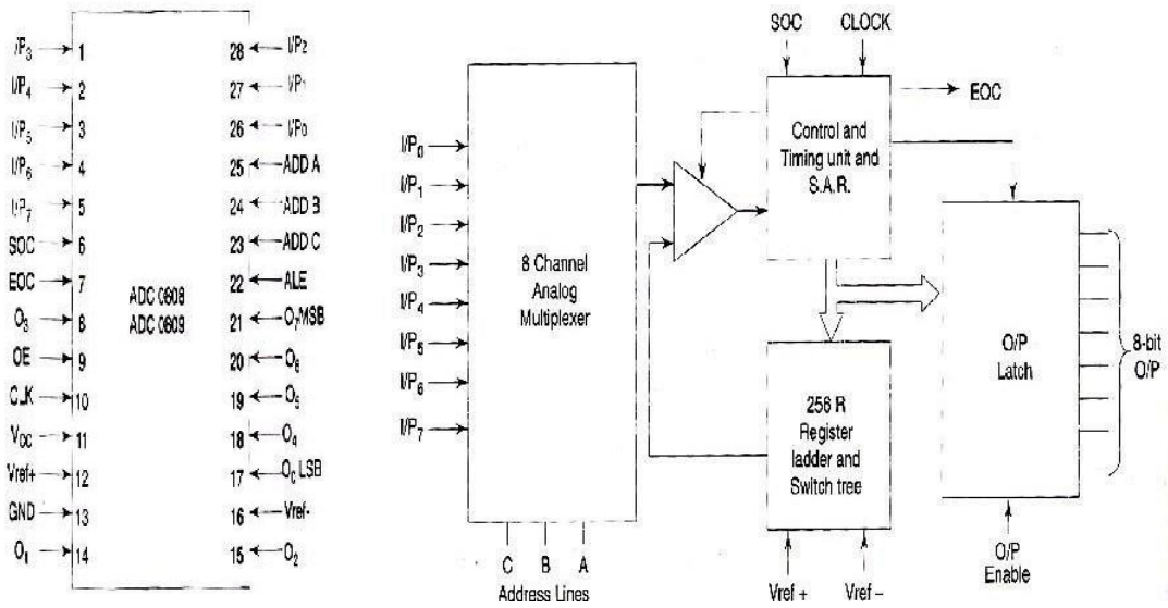
Fig. 3.21 Pins of ADC0808/09
