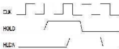
Bus request and bus grant timings in minimum
