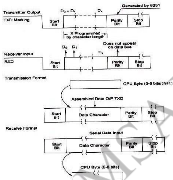
Fig. 3.17 communication format
