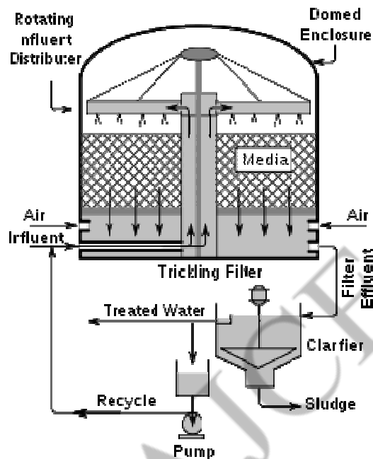
Trickling filter
