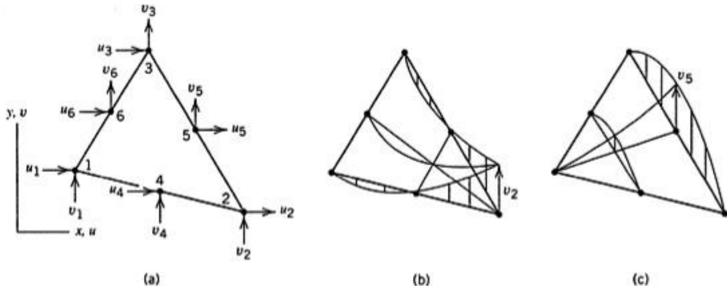
Fig. 3.3-1. (a) A linear strain triangle and its six nodal d.o.f. (b) Displacement mode associated with nodal d.o.f. v_2 . (c) Displacement mode associated with nodal d.o.f. v_5 . (For visualization only, imagine that displacement occurs normal to the plane of the element.) (b and c reprinted from [2.2] by permission of John Wiley & Sons, Inc.)
