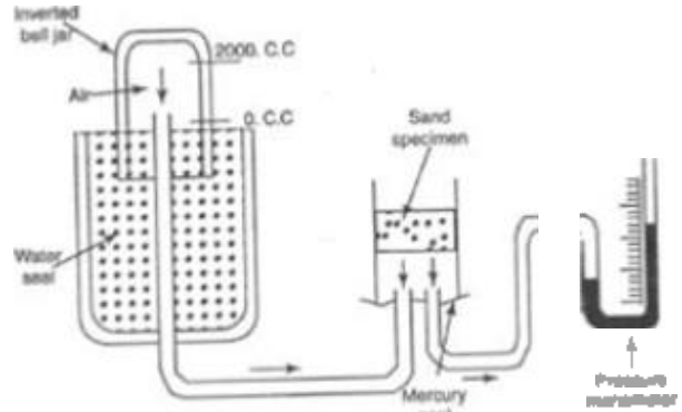
Fig. 1.16 Permeability Tester
