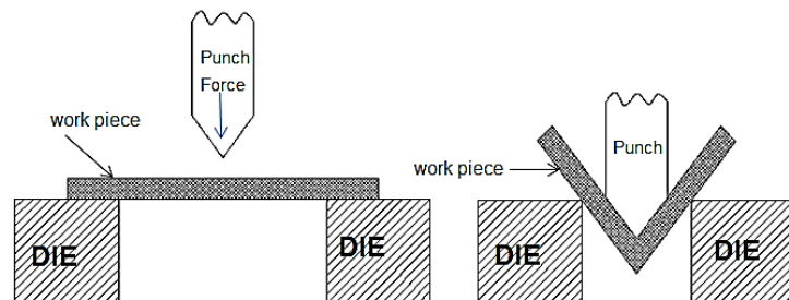
Air Bending
