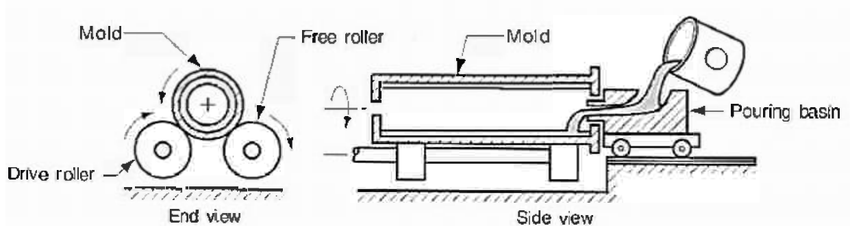
Fig. 1.40 Centrifugal casting
