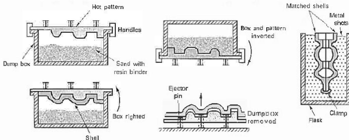
Fig.1.38 Step by step of shell moulding process
