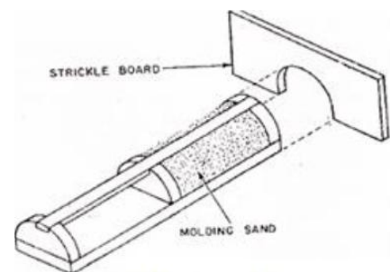
Fig. 1.8 Skeleton Pattern
