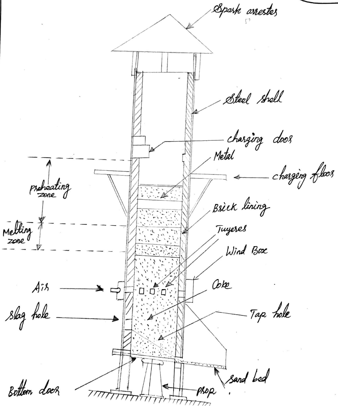
Figure cupola furnace
