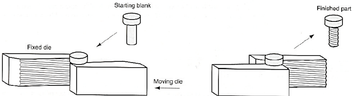
Fig. 3.30 Threading rolling with flat die
