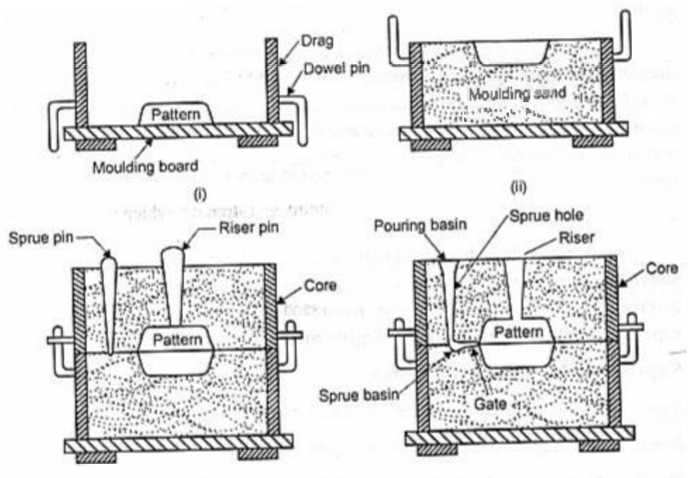
Fig. 1.31 Green sand Moulding Processes
