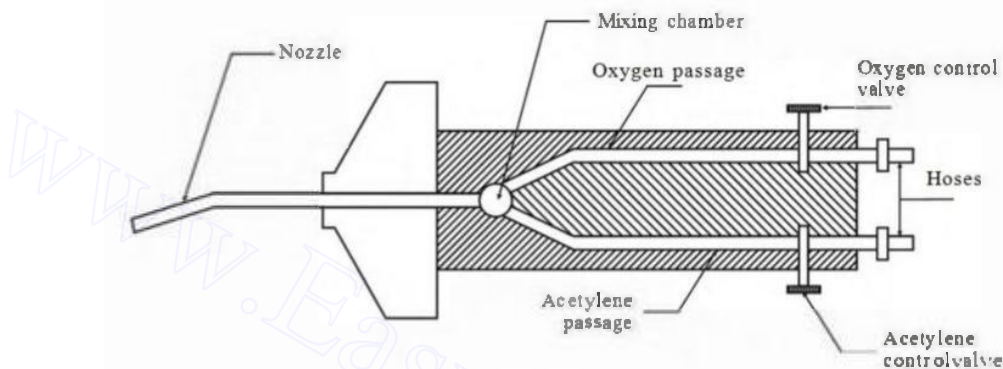
Fig.2.3 Welding Torch
