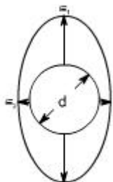
Fig 4.2 The relationship of major, e_1 , and minor, e_2 , strains is established by measurement after forming.
