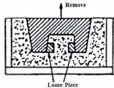
Fig. 1.5 Loose Piece Pattern
