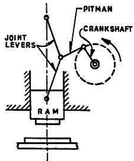
Fig.3.11: Knuckle Press
