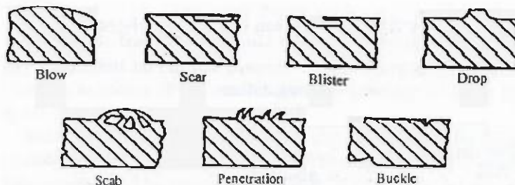
Fig. 1.48(a) Surface Defects
