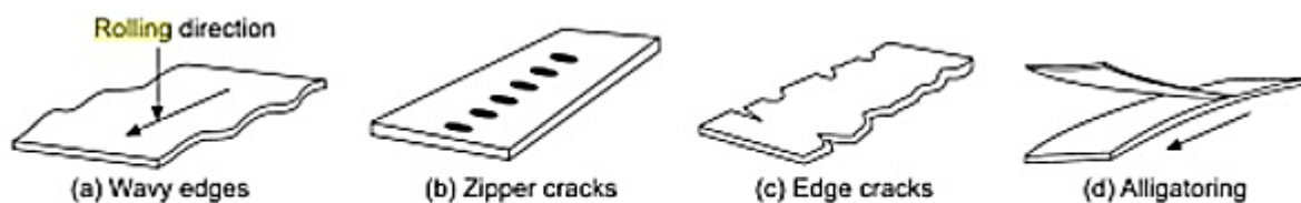
Fig. 3.31 Rolling defects
