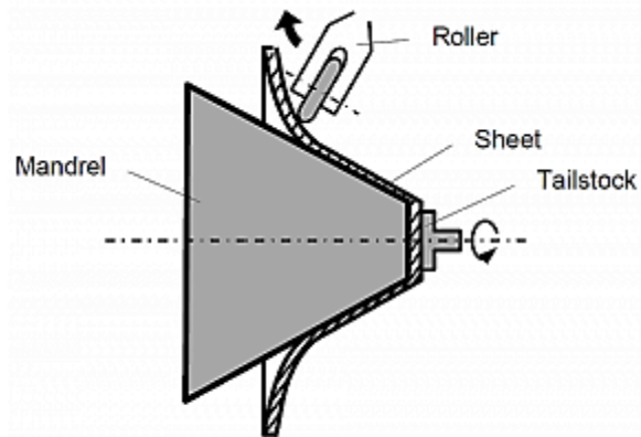
Metal Spinning
