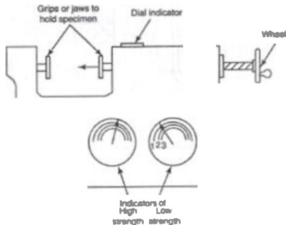
Fig.1.14 Strength Tester
