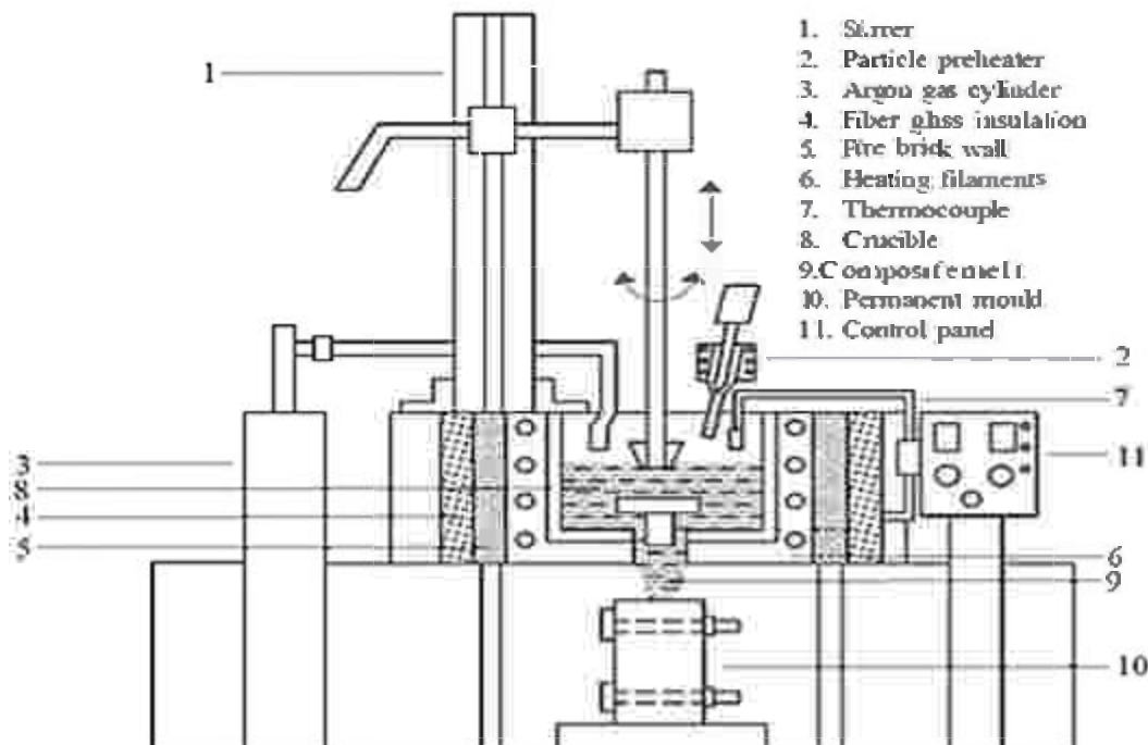
Fig. 1.46: Stir Casting
