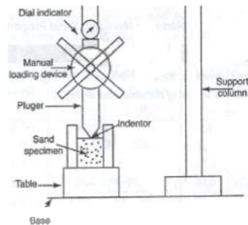
Fig. 1.17 Mold Hardness Tester
