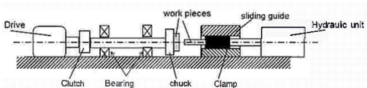
Fig.2.20 : Friction Welding
