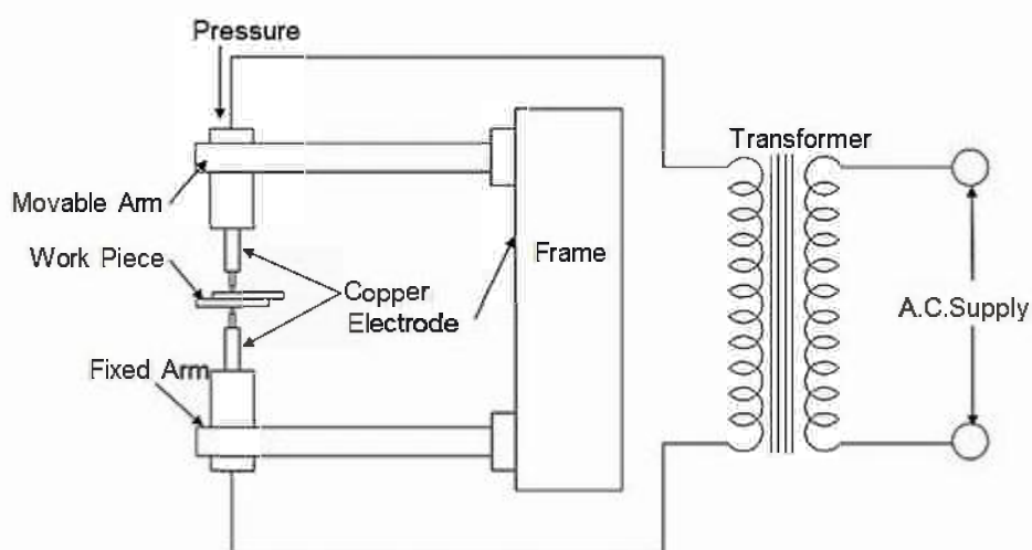
Fig. 2.10: Resistance welding
