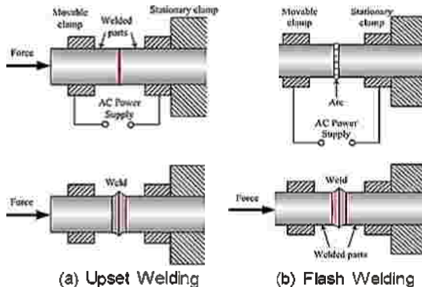
Fig. 2.11 Butt Welding
