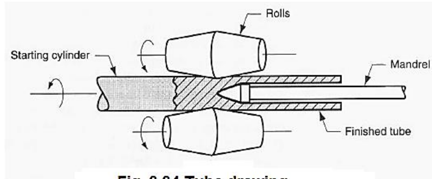
Fig. 3.34 Tube drawing (or) Tube Piercing (or) seamless tube drawing
