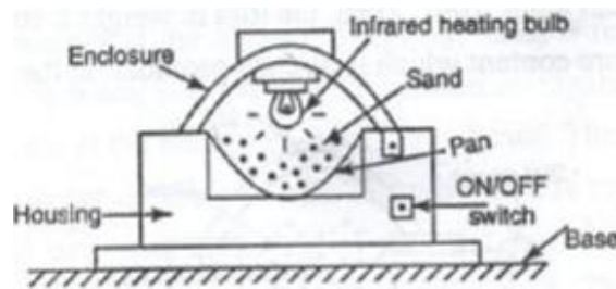
Fig.1.11 Evaporation method
