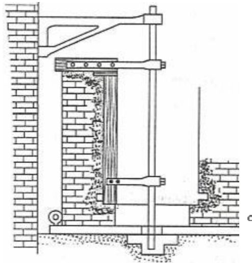
Fig.1.32 Loam Moulding with sweep pattern
