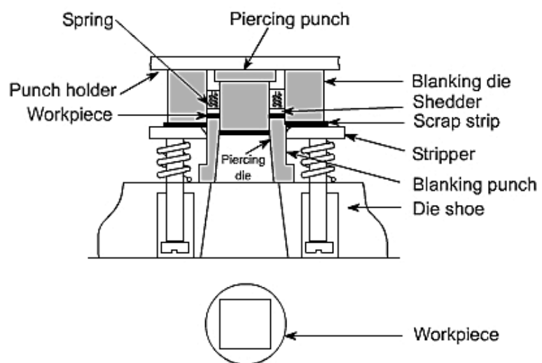
Compound Die
