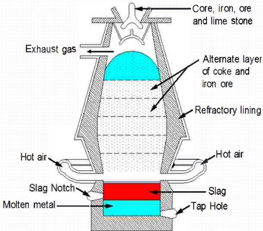
Fig.1.37: Blast Furnace
