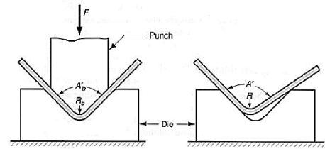
Springback in bending
