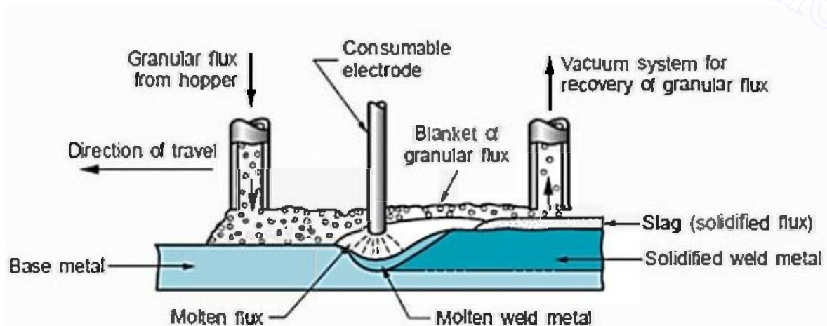
Fig.2.8 Submerged Arc Welding
