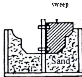
Fig.1.7 Sweep Pattern
