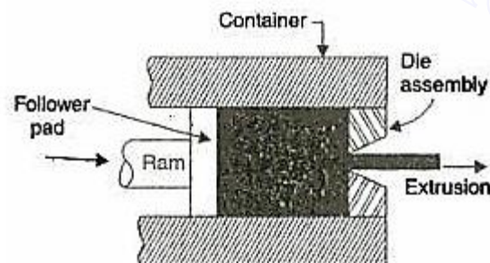
Fig. 3.36 Forward or Direct extrusion
