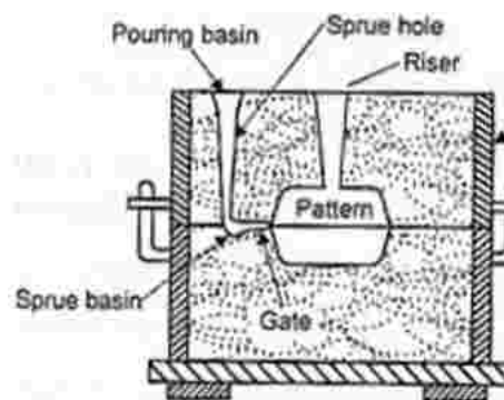
Fig.1.1 Method of sand casting
