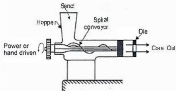
Fig.1.26 Core Extrusion Machine
