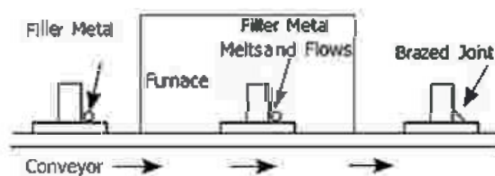
Fig.2.23 Furnace Brazing
