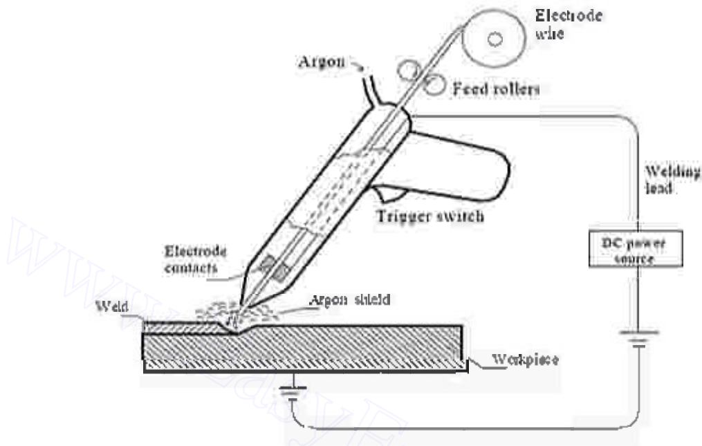
Fig.2.7 Metal Inert Gas (MIG) Welding
