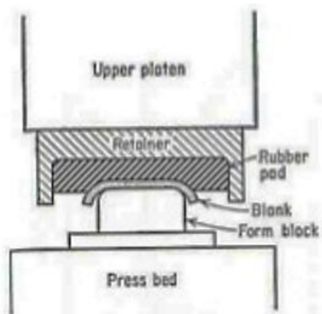
Rubber Pad Forming
