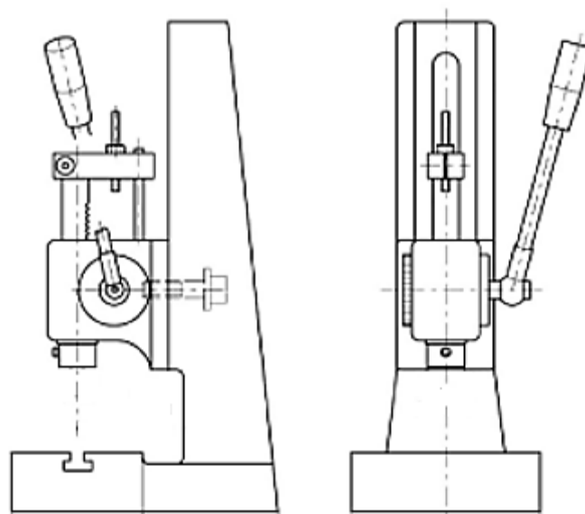
Fig. 3.14 Rack and Pinion Press
