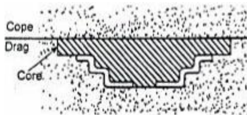
f) Cover core
