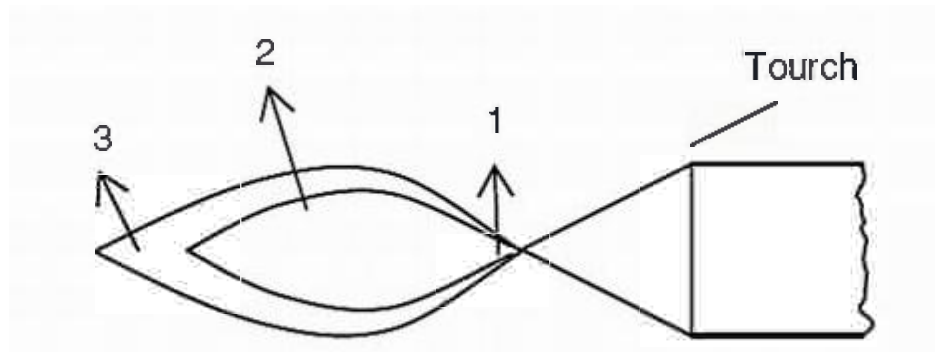
Fig.2.4 Flame establishment in oxy-acetylene welding
