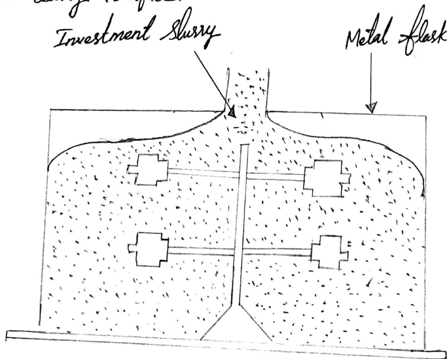
Figure Investment Casting with investment slurry.
