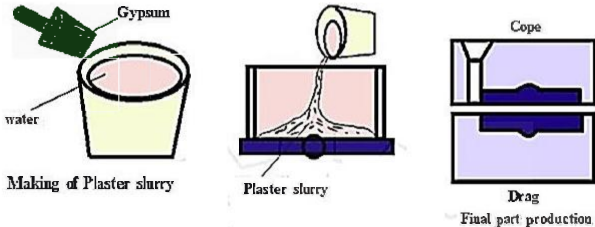
Fig.1.43 : Ceramic mould making
