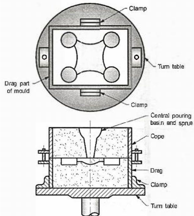
Fig.1.42 Centrifuge casting
