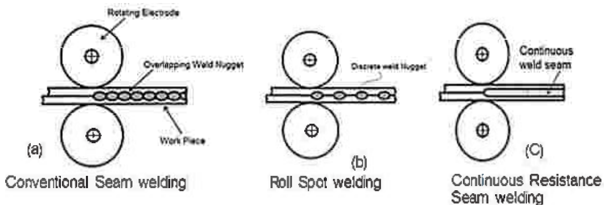
Fig.2.13 : Seam Welding
