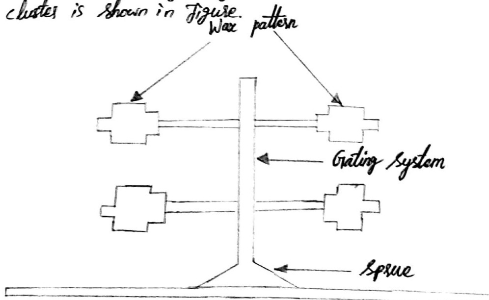
Figure Investment casting with gating system.
