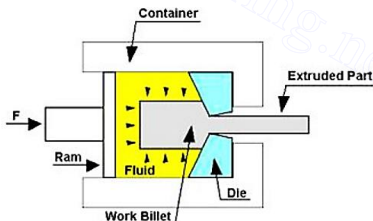
Fig. 3.40 Hydrostatic extrusion
