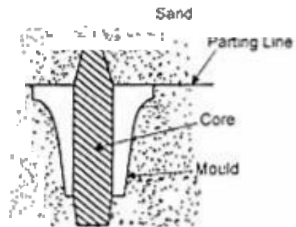
b) Vertical core
