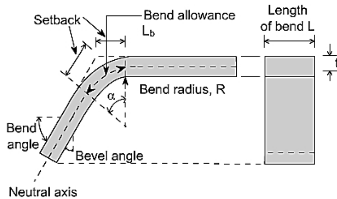
Bending Terminology
